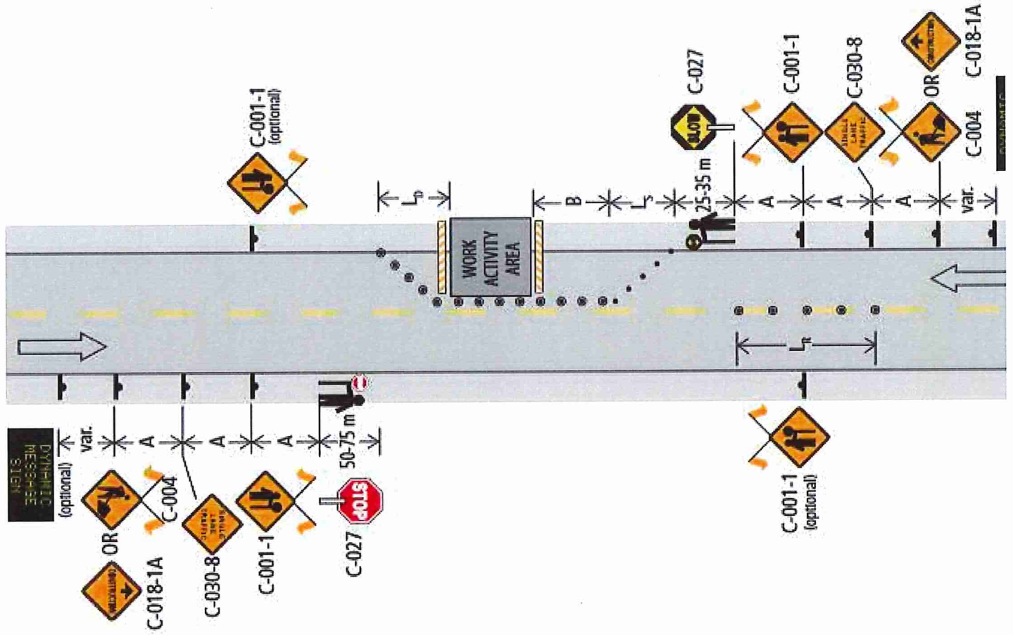
Figure 7.8: Lane Closure with TCPs – Single Lane Alternating – Short and Long Durations
